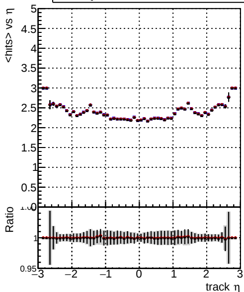
mean hits vs \eta Legend: DQM_V0001_R000000001_Global_mkFit_noCAND (blue), DQM_V0001_R000000001_Global_mkFit_CAND (red), DQM_V0001_R000000001_Global_mkFit_batchCAND (black)
