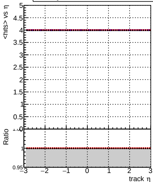
mean hits DQM_V0001_R000000001_Global_mkFit_noCAND DQM_V0001_R000000001_Global_mkFit_CAND DQM_V0001_R000000001_Global_mkFit_batchCAND
