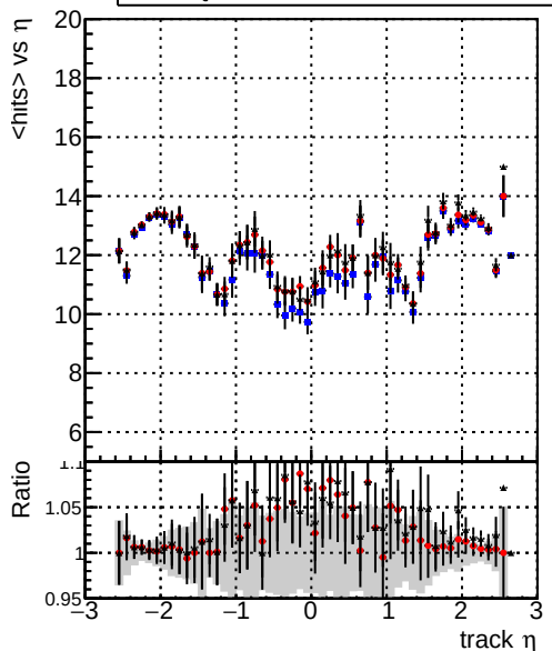
mean hits vs \eta Legend: DQM_V0001_R000000001_Global_mkFit_noCAND (blue line) DQM_V0001_R000000001_Global_mkFit_CAND (red line) DQM_V0001_R000000001_Global_mkFit_batchCAND (black line)
