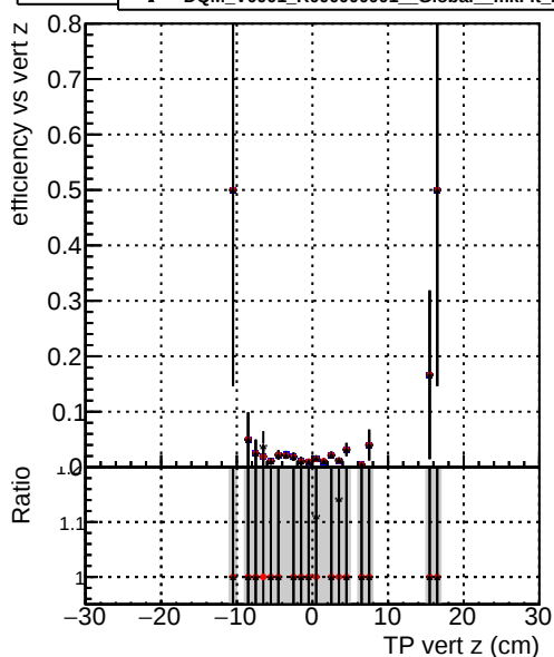
Efficiency vs vert z Global_mkFit_noCAND Global_mkFit_CAND Global_mkFit_batchCAND
