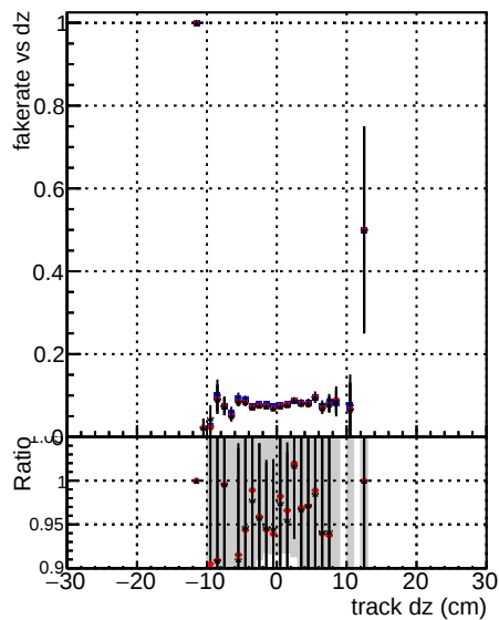
Fake rate vs d DOM V0001 R0000000001 Global mkFit noCAND DOM V0001 R0000000001 Global mkFit C-CAND DOM V0001 R0000000001 Global mkFit batchCAND
