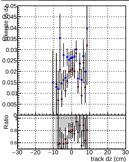
Legend Global mkFit noCAND Blue dots DOM V0001 R0000000001 Global Red dots DOM V0001 R0000000001 Global Black dots DOM V0001 R0000000001 Global Gray dots DOM V0001 R0000000001 Global
