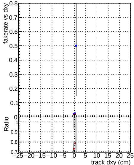
Legend Global mkFit noCAND Blue dots DOM V0001 R0000000001 Global Red dots DOM V0001 R0000000001 Global Black dots DOM V0001 R0000000001 Global Gray dots DOM V0001 R0000000001 Global
