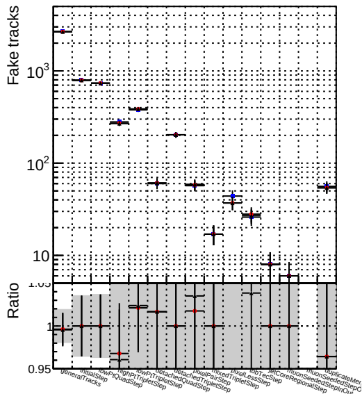
Number ● DQM_V0001_R0000000001_Global_mkFit_CAND ▲ DQM_V0001_R0000000001_Global_mkFit_batchCAND
