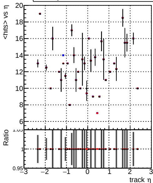
mean hit DQM_V0001_R000000001_Global_mkFit_noCAND DQM_V0001_R000000001_Global_mkFit_CAND DQM_V0001_R000000001_Global_mkFit_batchCAND
