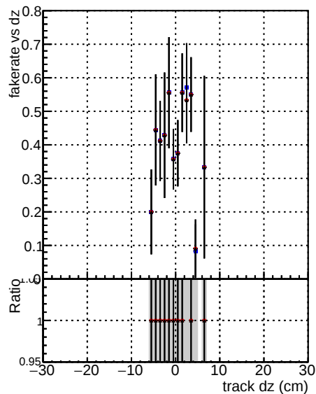
Fake rate vs dz Legend: DOM V0001 R0000000001 Global mkFit noCAND (Blue line with dots) DOM V0001 R0000000001 Global mkFit CAND (Red line with dots) DOM V0001 R0000000001 Global mkFit batchCAND (Black line with dots)
