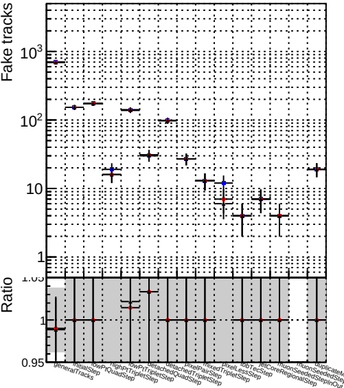
Number Legend ● DQM_V0001_R0000000001_Global_mkFit_CAND ▲ DQM_V0001_R0000000001_Global_mkFit_batchCAND
