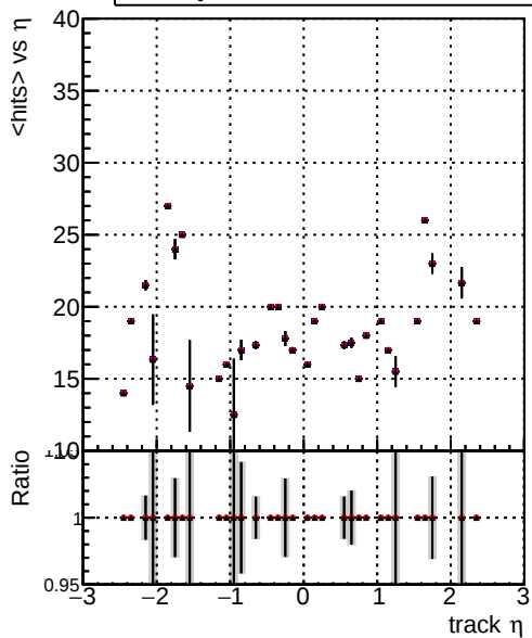
mean hit Legend: DQM_V0001_R000000001_Global_mkFit_noCAND (blue line) DQM_V0001_R000000001_Global_mkFit_CAND (red line) DQM_V0001_R000000001_Global_mkFit_batchCAND (black line)
