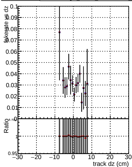
Fake rate vs d DOM V0001 R0000000001 Global mkFit noCAND DOM V0001 R0000000001 Global mkFit batchCAND
