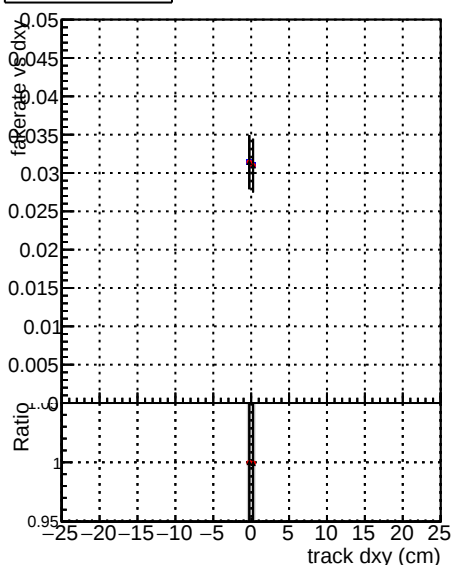
Fake rate vs d DOM V0001 R0000000001 Global mkFit noCAND DOM V0001 R0000000001 Global mkFit batchCAND
