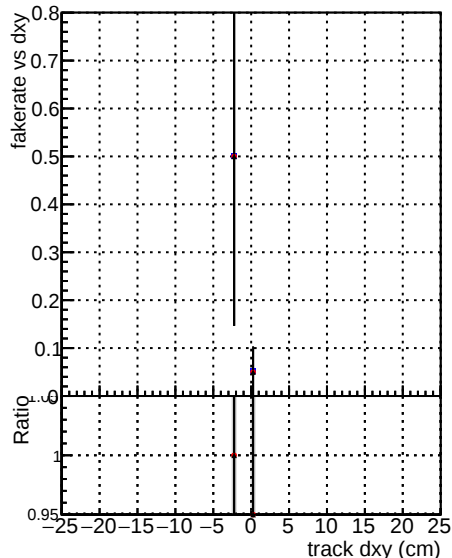
Legend for Fake rate vs dxy and Duplicates Rate vs Dxy plots: DOM V0001 R0000000001 Global mkFit noCAND DOM V0001 R0000000001 Global mkFit CAND DOM V0001 R0000000001 Global mkFit batchCAND
