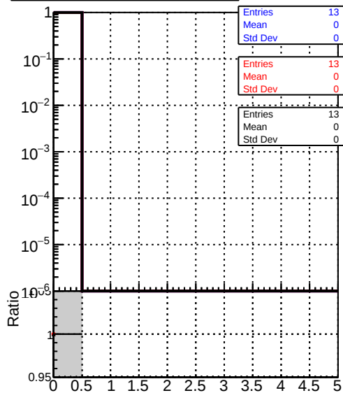
mean hit DQM_V0001_R000000001_Global_mkFit_noCAND DQM_V0001_R000000001_Global_mkFit_CAND DQM_V0001_R000000001_Global_mkFit_batchCAND
