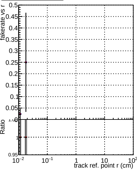
Legend: DQM_V0001_R000000001 Global mkFit_noCAND, DQM_V0001_R000000001 Global mkFit_CAND, DQM_V0001_R000000001 Global mkFit_batchCAND
