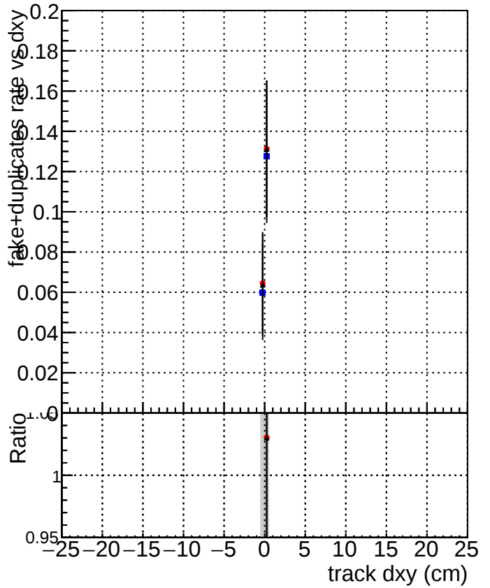
DQM_V0001_R000000001_Global_mkFit_noCAND DQM_V0001_R000000001_Global_mkFit_CAND DQM_V0001_R000000001_Global_mkFit_batchCAND
