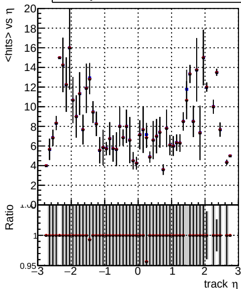
mean hits DQM_V0001_R0000000001_Global_mkFit_noCAND DQM_V0001_R0000000001_Global_mkFit_CAND DQM_V0001_R0000000001_Global_mkFit_batchCAND
