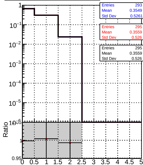
mean hits DQM_V0001_R0000000001_Global_mkFit_noCAND DQM_V0001_R0000000001_Global_mkFit_CAND DQM_V0001_R0000000001_Global_mkFit_batchCAND
