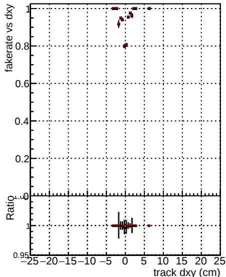
Global mkFit noCAND Global mkFit CAND Global mkFit batchCAND
