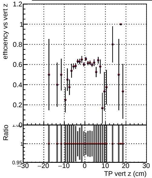
Efficiency vs. TP vert z (cm) —●— DQM_V0001_R0000000001_Global_mkFit_noCAND —●— DQM_V0001_R0000000001_Global_mkFit_CAND —●— DQM_V0001_R0000000001_Global_mkFit_batchCAND
