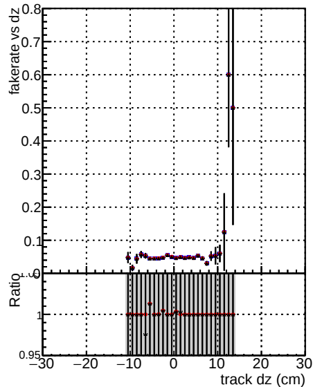
DOM V0001 R0000000001 Global mkFit noCAND DOM V0001 R0000000001 Global mkFit batchCAND
