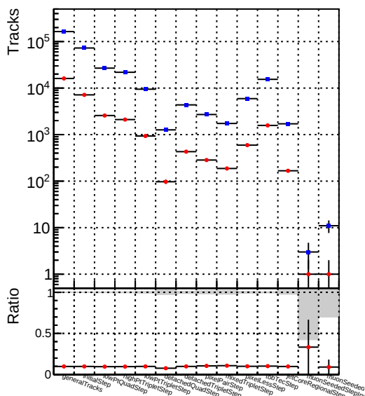
■ DQM_V0001_R000000001 Global mkFit baseline
