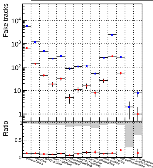
Number DOM V0001 R0000000001 Global mkFit var
