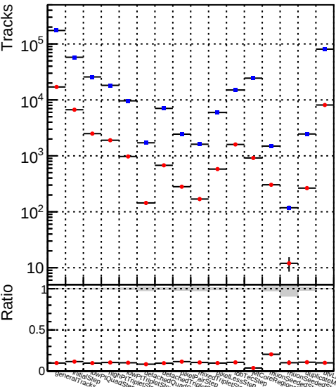
DQM_V0001_R000000001_Global_mkFit_baseline
