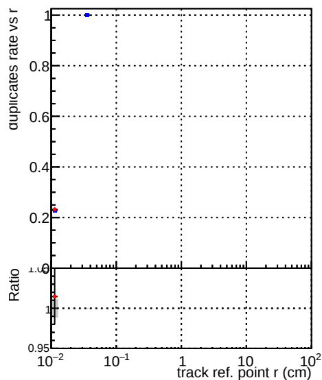
—•— DQM_V0001_R000000001_Global_mkFit_baseline —•— DQM_V0001_R000000001_Global_mkFit_var
