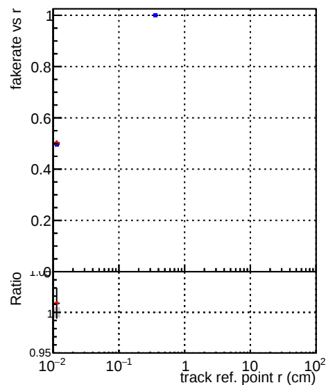
—•— DQM_V0001_R000000001_Global_mkFit_baseline —•— DQM_V0001_R000000001_Global_mkFit_var
