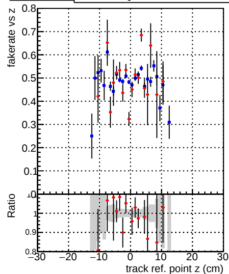
—•— DQM_V0001_R000000001_Global_mkFit_baseline —•— DQM_V0001_R000000001_Global_mkFit_var
