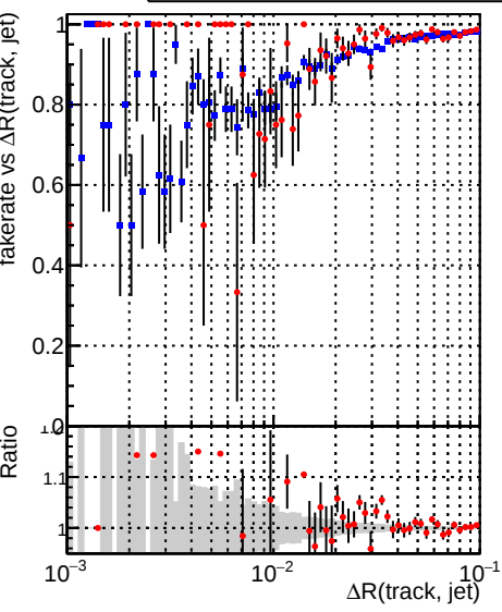
Legend: DQM_V0001_R000000001_Global_mkFit_baseline (blue squares), DQM_V0001_R000000001_Global_mkFit_var (red circles)
