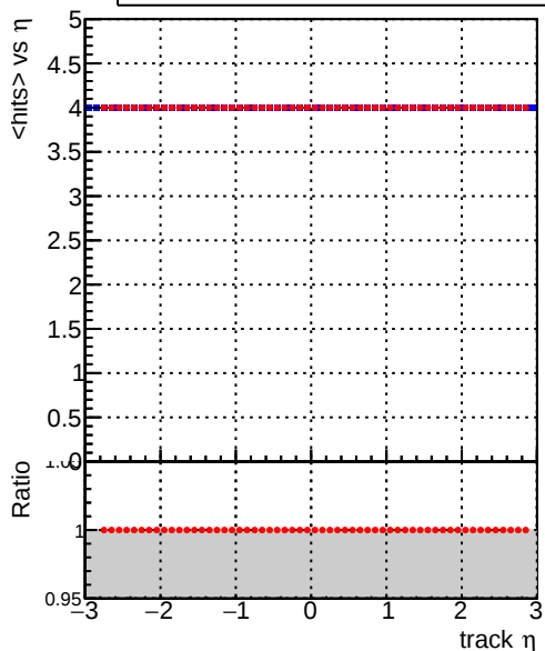
mean hits — DQM_V0001_R000000001_Global_mkFit_baseline — DQM_V0001_R000000001_Global_mkFit_var
