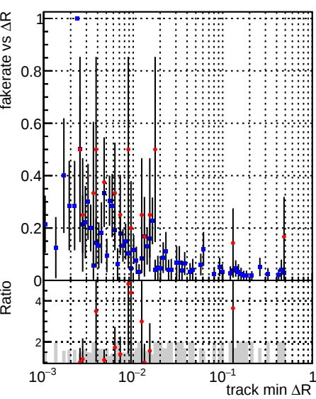
Legend: DQM_V0001_R000000001_Global_mkFit_baseline (blue dots), DQM_V0001_R000000001_Global_mkFit_var (red dots)
