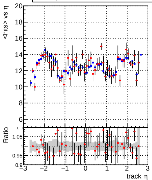
DQM_V0001_R000000001_Global_mkFit_var
