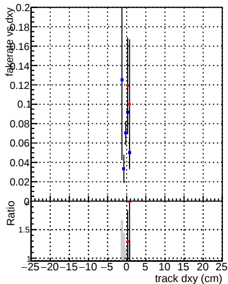
—●— DQM_V0001_R0000000001_Global_mkFit_baseline —●— DQM_V0001_R0000000001_Global_mkFit_var
