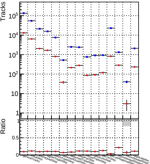
DQM_V0001_R000000001_Global_mkFit_baseline
