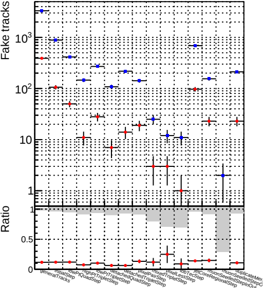
Number —●— DQM_V0001_R000000001_Global_mkFit_var
