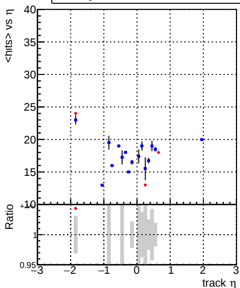
mean hits vs \eta Legend: DQM_V0001_R000000001_Global_mkFit_baseline (blue line), DQM_V0001_R000000001_Global_mkFit_var (red line)
