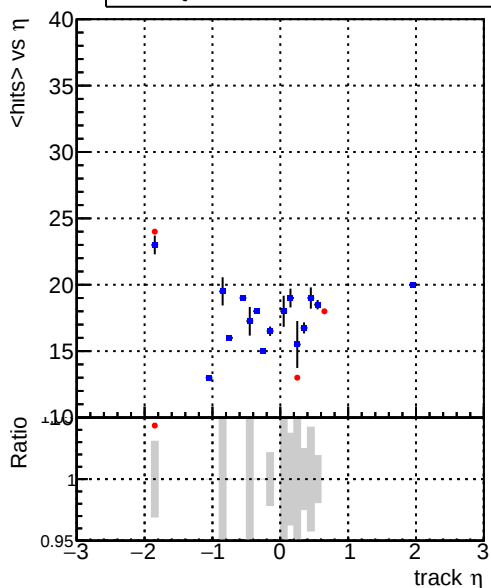
mean hits vs \eta — DQM_V0001_R000000001_Global_mkFit_baseline — DQM_V0001_R000000001_Global_mkFit_var
