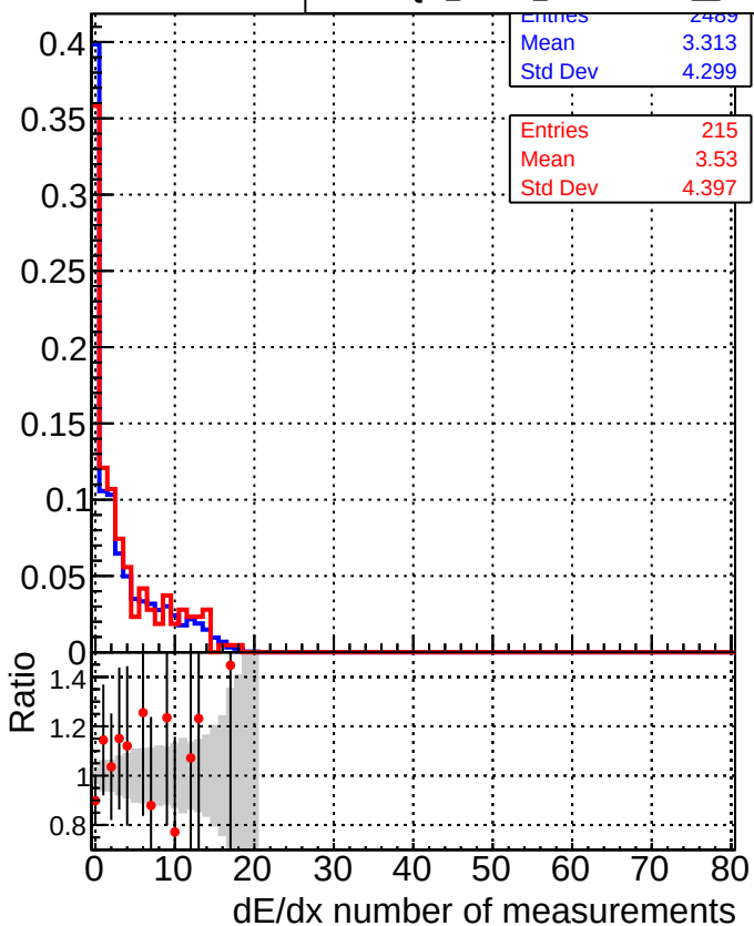
■ DQM_V0001_R000000001_Global_mkFit_baseline ● DQM_V0001_R000000001_Global_mkFit_var
