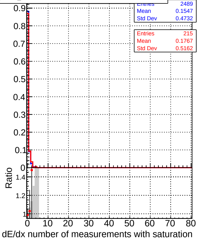
■ DQM_V0001_R000000001_Global_mkFit_baseline ● DQM_V0001_R000000001_Global_mkFit_var
