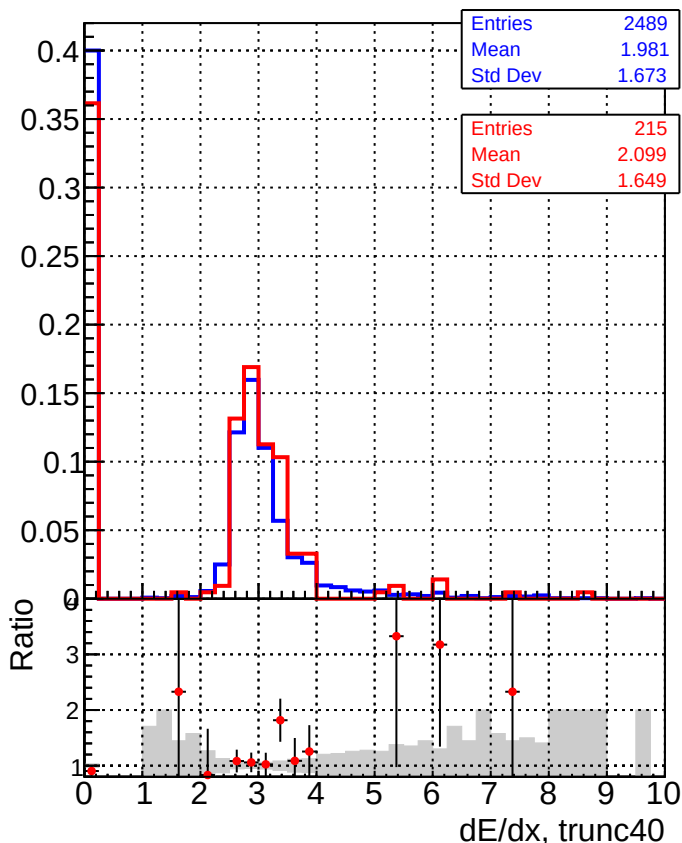
■ DQM_V0001_R000000001_Global_mkFit_baseline ● DQM_V0001_R000000001_Global_mkFit_var
