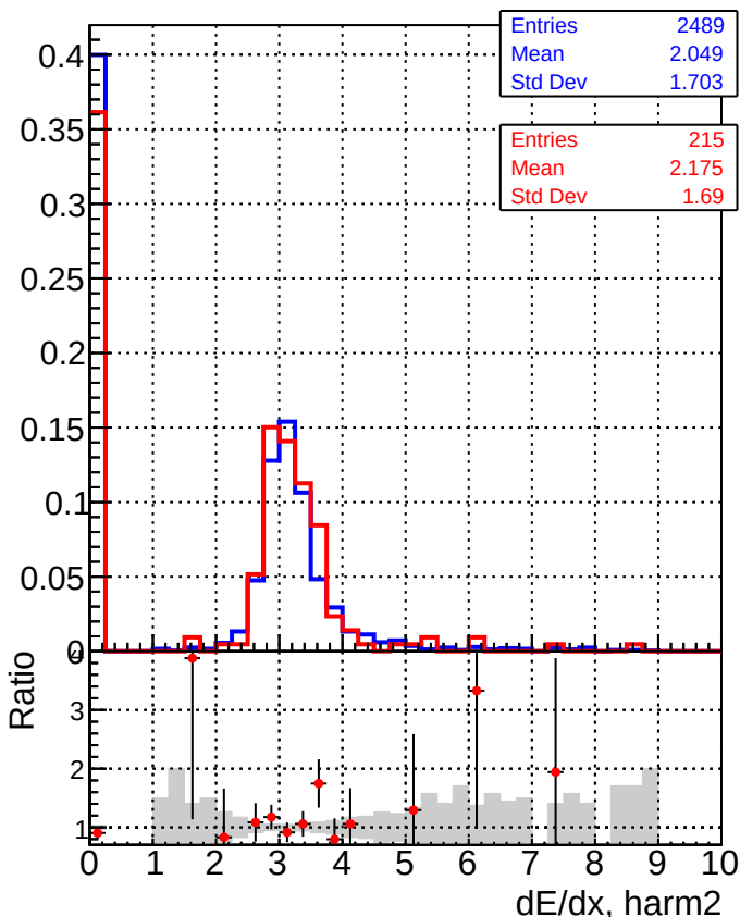
■ DQM_V0001_R000000001_Global_mkFit_baseline ● DQM_V0001_R000000001_Global_mkFit_var
