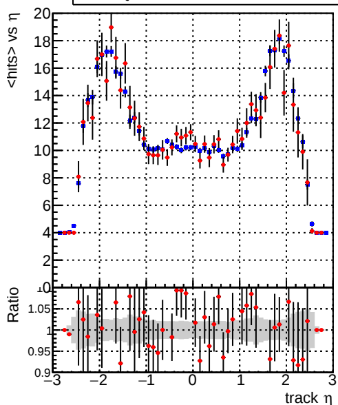
— DQM_V0001_R000000001_Global_mkFit_baseline — DQM_V0001_R000000001_Global_mkFit_var
