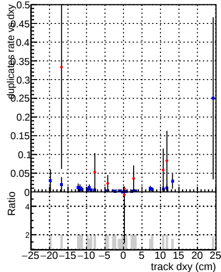
—●— DQM_V0001_R0000000001_Global_mkFit_baseline —●— DQM_V0001_R0000000001_Global_mkFit_var
