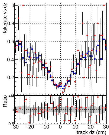
—●— DQM_V0001_R0000000001_Global_mkFit_baseline —●— DQM_V0001_R0000000001_Global_mkFit_var
