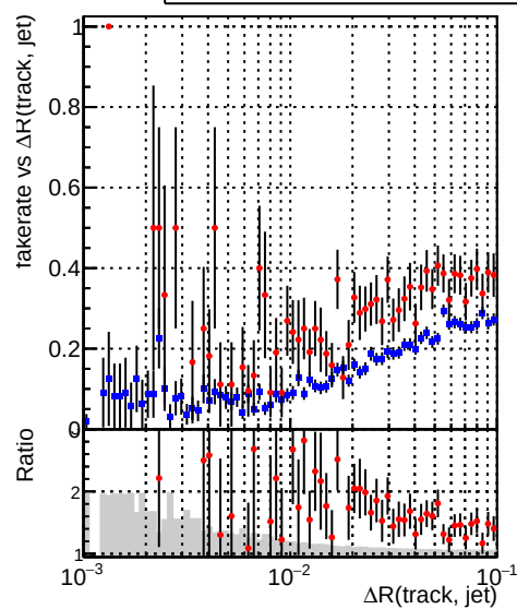
—●— DQM_V0001_R000000001_Global_mkFit_baseline —●— DQM_V0001_R000000001_Global_mkFit_var
