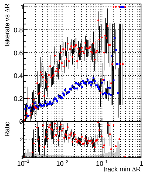
—●— DQM_V0001_R000000001_Global_mkFit_baseline —●— DQM_V0001_R000000001_Global_mkFit_var
