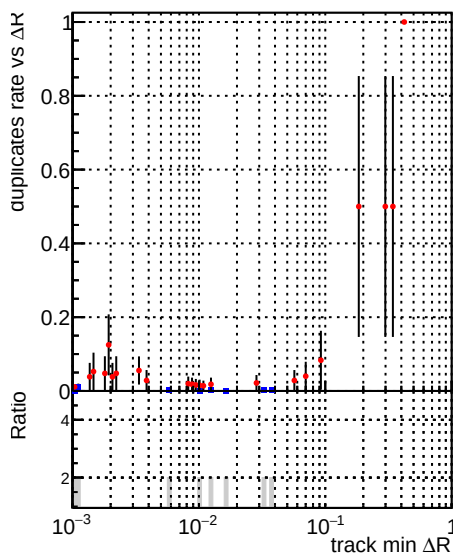
—●— DQM_V0001_R000000001_Global_mkFit_baseline —●— DQM_V0001_R000000001_Global_mkFit_var
