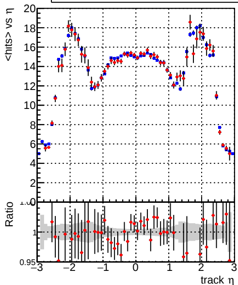
mean hits vs \eta — DQM_V0001_R000000001_Global_mkFit_baseline — DQM_V0001_R000000001_Global_mkFit_var
