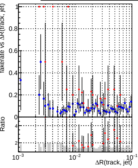
Fake rate vs \Delta R(\text{track, jet}) Legend: —●— DQM_V0001_R000000001_Global_mkFit_baseline —●— DQM_V0001_R000000001_Global_mkFit_var
