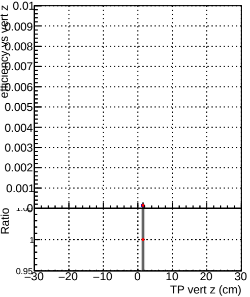
Efficiency vs TP vert z (cm) Legend: DQM_V0001_R0000000001_Global_mkFit_baseline DQM_V0001_R0000000001_Global_CMSSW_X_Y_Z_RECO
