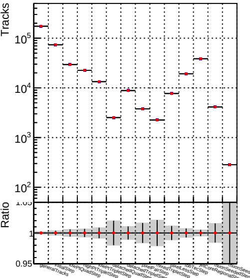
■ DQM_V0001_R000000001_Global_mkFit_baseline
