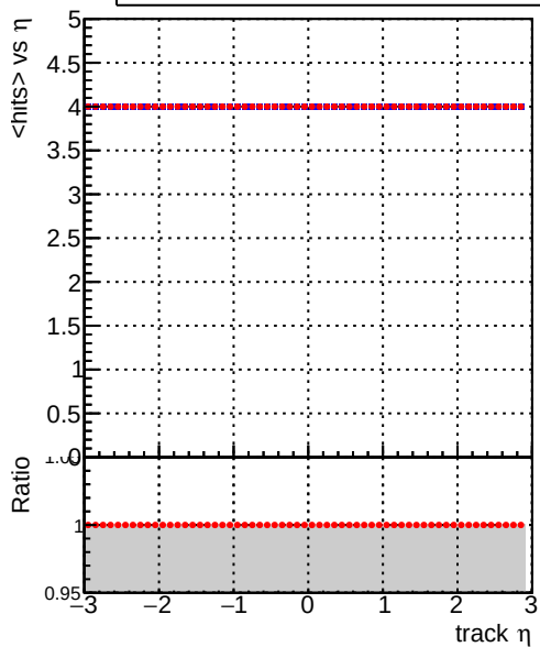
mean hits Legend: DQM_V0001_R000000001_Global_mkFit_baseline (blue line), DQM_V0001_R000000001_Global_CMSSW_X_Y_Z_RECO (red line)
