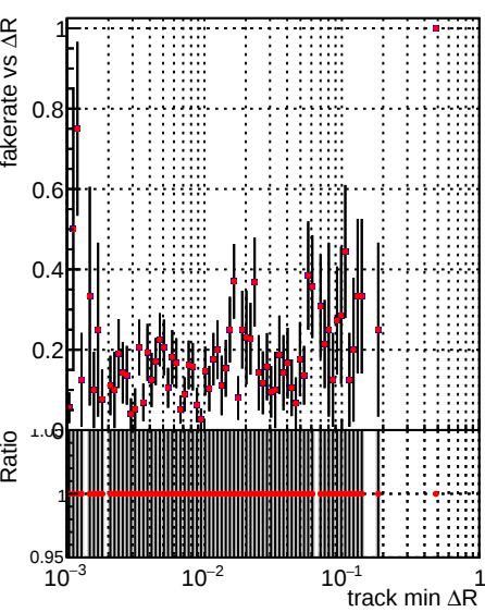
Fake rate vs \Delta R(\text{track, jet}) DQM_V0001_R000000001_Global_mkFit_baseline DQM_V0001_R000000001_Global_CMSSW_X_Y_Z_RECO
