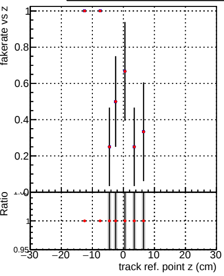
Fake rate vs v Legend: - DQM_V0001_R000000001_Global_mkFit_baseline (gray line with error bars) - DQM_V0001_R000000001_Global_CMSSW_X_Y_Z_RECO (red line with error bars)
