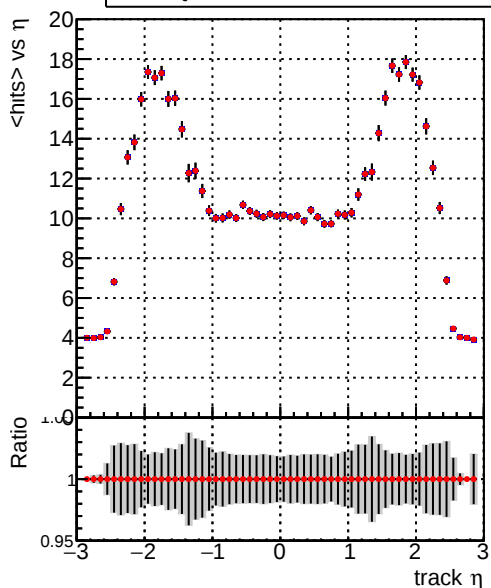
— DQM_V0001_R000000001_Global_mkFit_baseline — DQM_V0001_R000000001_Global_CMSSW_X_Y_Z_RECO
