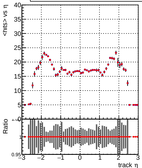
mean hits vs \eta Legend: DQM_V0001_R000000001_Global_mkFit_baseline (blue line), DQM_V0001_R000000001_Global_CMSSW_X_Y_Z_RECO (red line)
