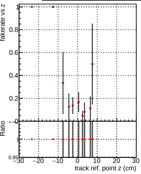
Fake rate vs verpos Legend: DQM_V0001_R000000001_Global_mkFit_baseline DQM_V0001_R000000001_Global_CMSSW_X_Y_Z_RECO
