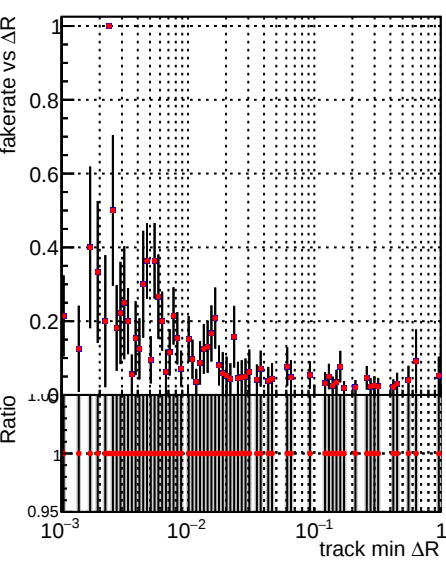
Fake rate vs \Delta R(\text{track, jet}) Legend: DQM_V0001_R000000001_Global_mkFit_baseline (black line with error bars) DQM_V0001_R000000001_Global_CMSSW_X_Y_Z_RECO (red line)
