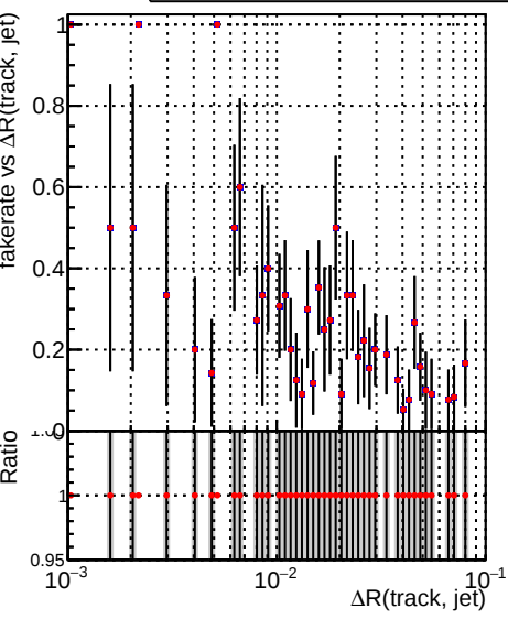
Fake rate vs \Delta R(\text{track, jet}) Legend: DQM_V0001_R000000001_Global_mkFit_baseline (black line with error bars) DQM_V0001_R000000001_Global_CMSSW_X_Y_Z_RECO (red line)
