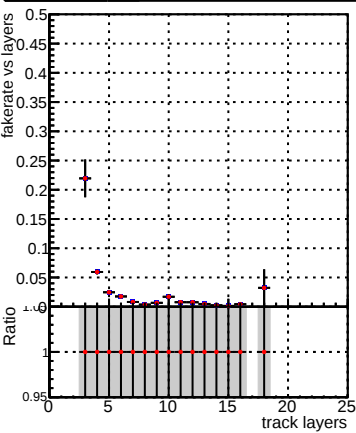
Legend: DQM_V0001_R000000001_Global_mkFit_baseline (grey shaded area), DQM_V0001_R000000001_Global_CMSSW_X_Y_Z_RECO (red dots with error bars)
