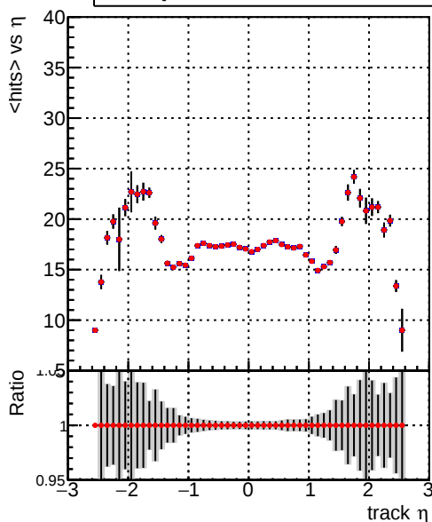
mean hit — DQM_V0001_R000000001_Global_mkFit_baseline — DQM_V0001_R000000001_Global_CMSSW_X_Y_Z_RECO
