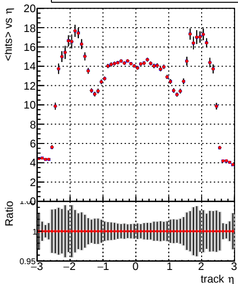
mean hit — DQM_V0001_R000000001_Global_mkFit_baseline — DQM_V0001_R000000001_Global_CMSSW_X_Y_Z_RECO
