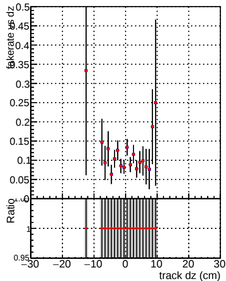
Fake rate vs dz —●— DQM_V0001_R0000000001_Global_mkFit_baseline —●— DQM_V0001_R0000000001_Global_CMSSW_X_Y_Z_RECO
